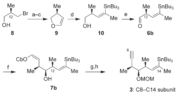
Scheme 3. Synthesis of the C8–C14 subunit 3 . a) NaCN, DMSO, 60 °C, 24 h, 92 %; b) DIBAL-H, \text{CH}_2\text{Cl}_2 , –78 °C, 2 h, 82 %; c) p -TSA (0.2 mol %), quinoline, 160 → 210 °C, 30 min, 85 %; d) t BuLi, \text{Me}_2\text{CuLi}_2\cdot\text{LiCN} , \text{Et}_2\text{O}/\text{DMS} (4:1), 0 °C → RT, 18 h, then n\text{Bu}_3\text{SnCl} , –20 °C → RT, 4 h, 68 %; e) TEMPO (10 mol %), \text{PhI}(\text{OAc})_2 , \text{CH}_2\text{Cl}_2 , RT, 2 h; f) 5 , pentane/cyclohexane, –78 °C, 3 h, 84 % (two steps); g) t BuLi, \text{Et}_2\text{O} , –40 → –20 °C, 20 min, 78 %; h) MOMCl, TBAI, Hünig's base, \text{CH}_2\text{Cl}_2 , 18 h, 92 %. DIBAL-H = diisobutylaluminum hydride, p -TSA = p -toluenesulfonic acid, DMS = dimethyl sulfide, TEMPO = 2,2,6,6-tetramethyl-1-piperidinyloxy free radical, MOM = methoxymethyl, TBAI = tetra- n -butylammonium iodide, Hünig's base = diisopropylethylamine.
